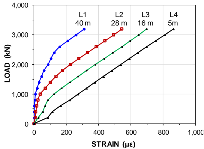
Fig. 8.74 Strains measured for the applied loads.
