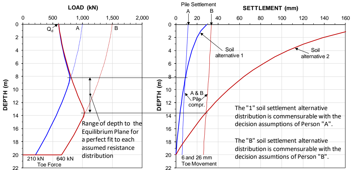
Fig. 8.88 Force distributions as deduced by Persons A and B
