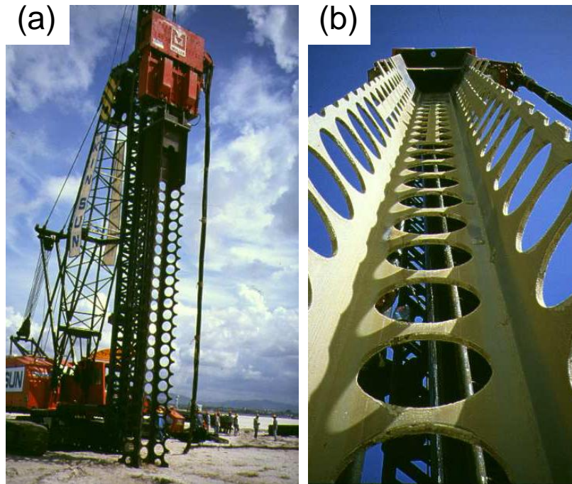
Fig. 10.10. Resonance compaction system, MRC, a system that uses a variable-frequency vibrator and a flexible (low axial stiffness) compaction probe.
