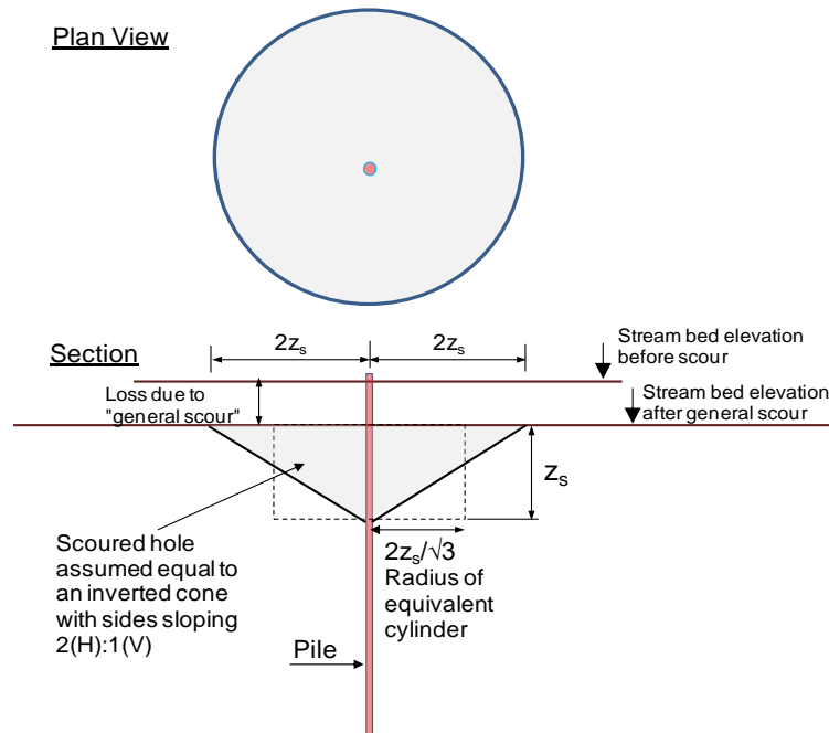
Fig. 7.63 Scour configuration according to the FHWA Manual
