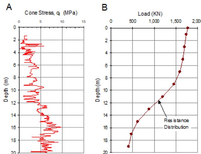
Fig. 8.42 A: CPT profile. B: CAPWAP determined load-distribution.
