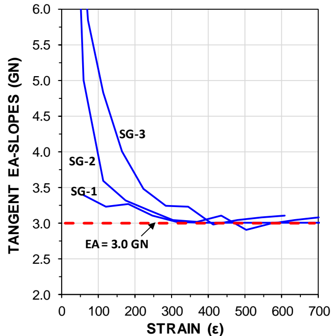
Fig. 3 EA-parameter by the tangent method
