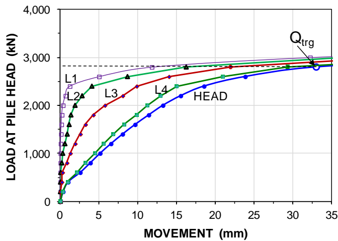
Fig. 8.75 Movements measured for the applied loads Q_{trg} = \text{Target Load} .
