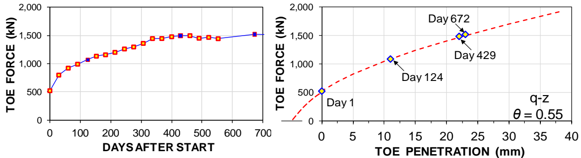
Fig. 7.21A Toe force vs. days after start
