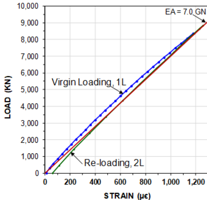
Fig. 8.64 Load-strain plot for virgin loading and re-loading with approximate stiffness line ( EA/L = 7.0 GN/m).
