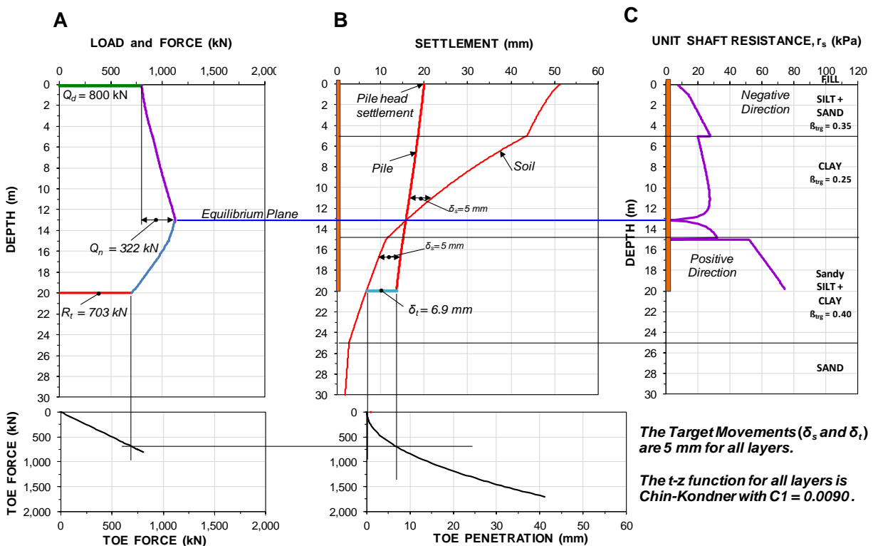
Fig. 2 Single pile after placing the fill. Unified Method results
