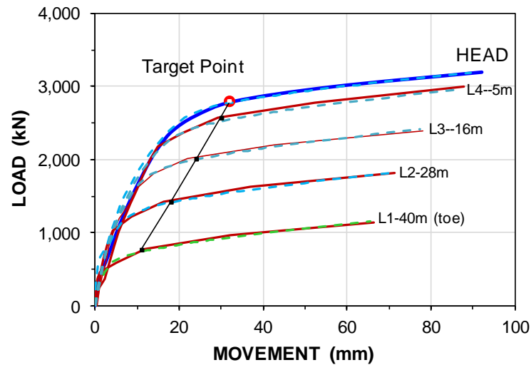
Fig. 8.85 Measured and fitted load-movement curves of pile head and gage levels
