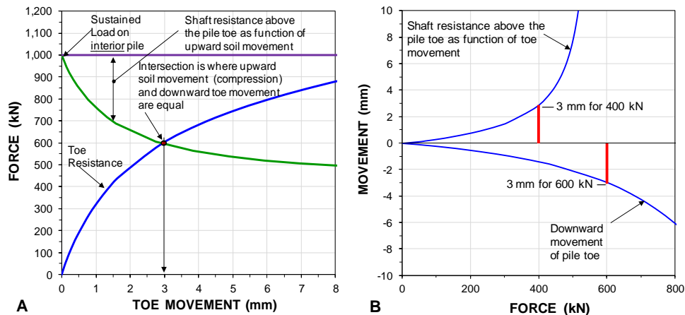
Fig. 7.36. The process for determining the load-transfer toe-movement for interior piles.
