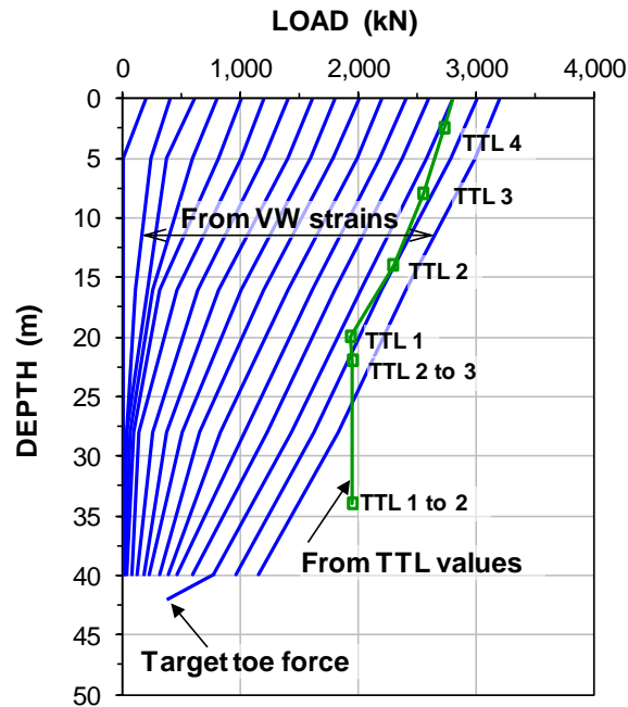
Fig. 8.80 Force distributions at VW-gages and from telltales at the 2,800-kN Target Load
