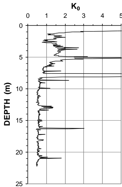
Fig. 2.24 K_0 profile determined from the CPTU sounding. Data from Paddle River site, Alberta (Fellenius 2006).
