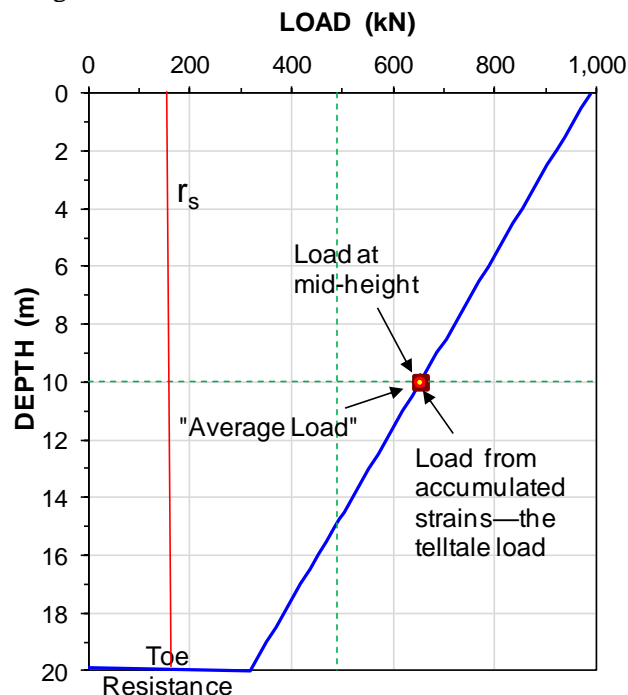
Fig. 8.20 Force distribution for constant unit shaft resistance.
