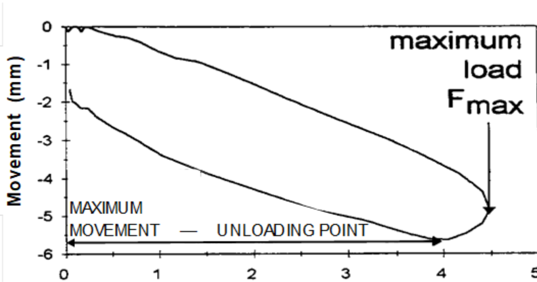
Fig. 9.21 Load-movement curve from Statnamic test (Bermingham et al. 1993)
