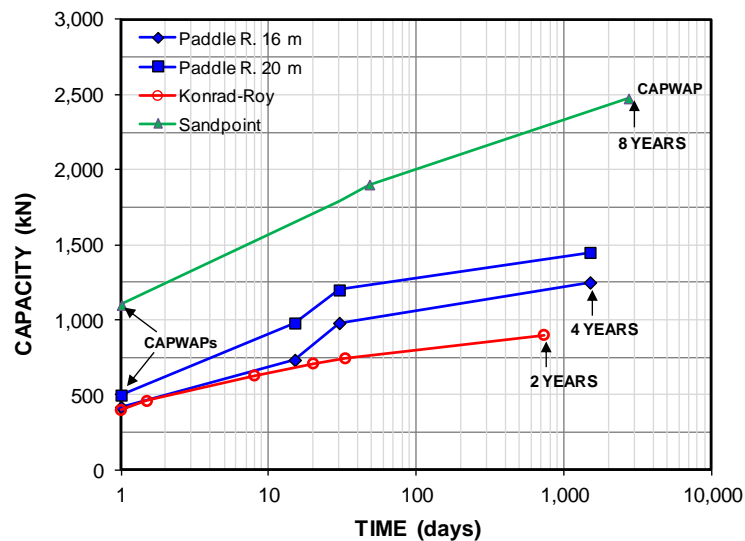
Fig. 7.61 "Capacity" determined at days after driving
