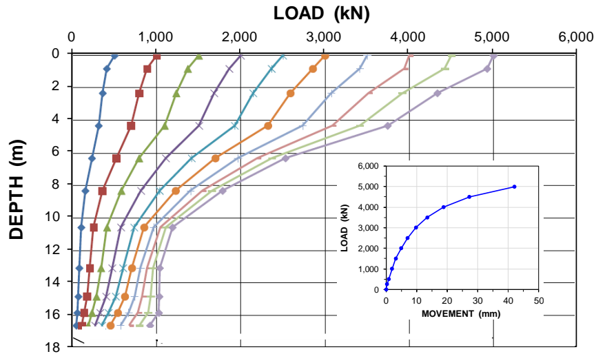
Fig. 8.32. Load distribution for a 620 mm diameter, 16.6 m long screw pile (Burlon 2016).
