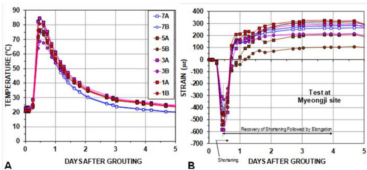
Fig. 8.40 Development of temperature and strain in a 35 m long spun-pile pile during first 5 days after grouting (reducing strain indicates compression/shortening) (Fellenius et al. 2009).
