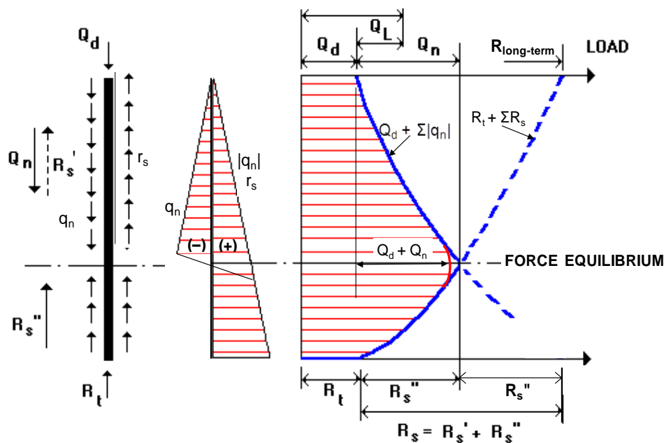
Fig. 7.23 Construing the Force Equilibrium
