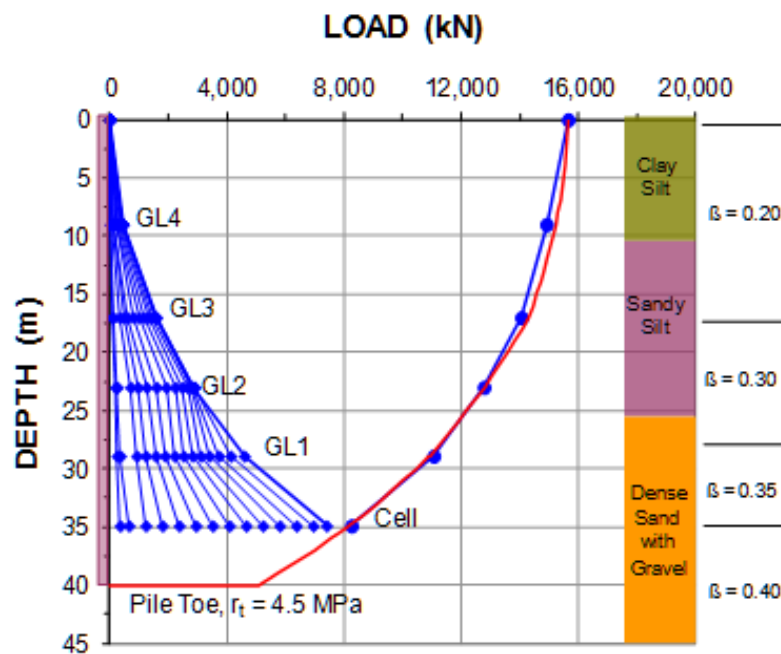
Fig. 8.28 Measured load distribution and the equivalent head-down load-distribution for the last maximum cell load ( r_t = \text{toe resistance} ).
