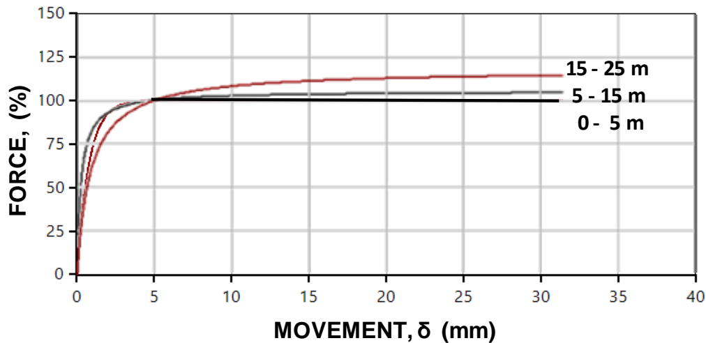
Fig. 5 t-z curves assigned to the preparation of the example
