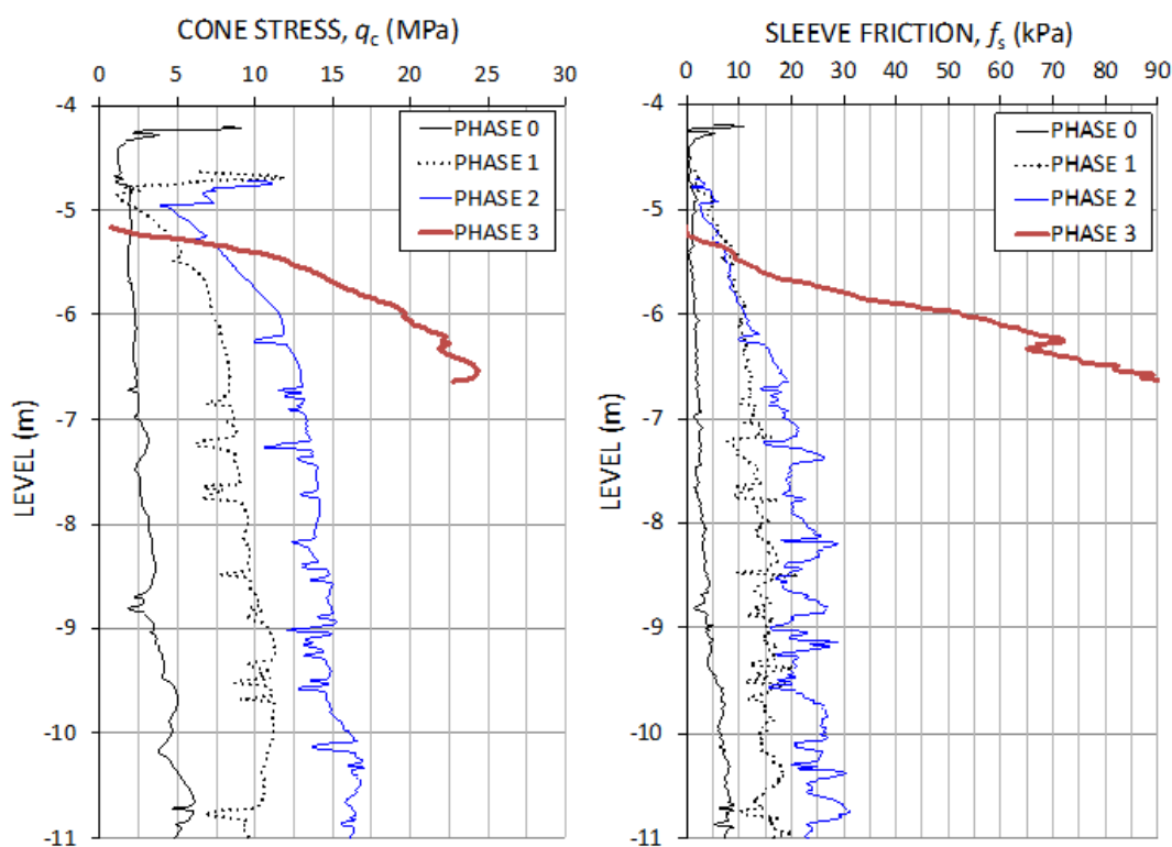
Fig. 10.31 Cone stress and sleeve friction from prior to compaction, and after each compaction phase.
