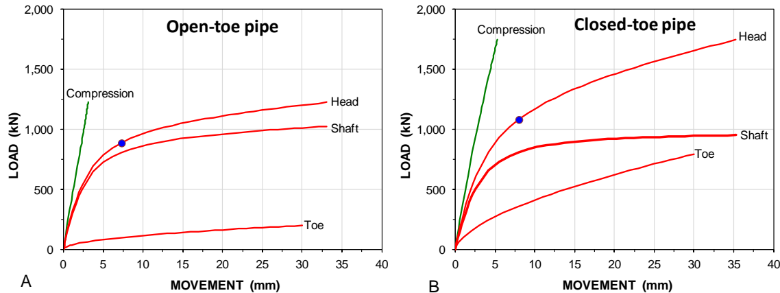
Fig. 7.53 Load-movement curves for a static loading test on (A) open-toe and (B) closed-toe piles
