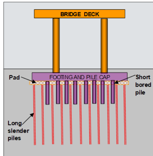
Fig. 7.47 Piled pad foundations for the Golden Ears Bridge piers. The short bored piles carry lateral forces, the long slender piles carry the structure (after Sampaco et al. 2008)
