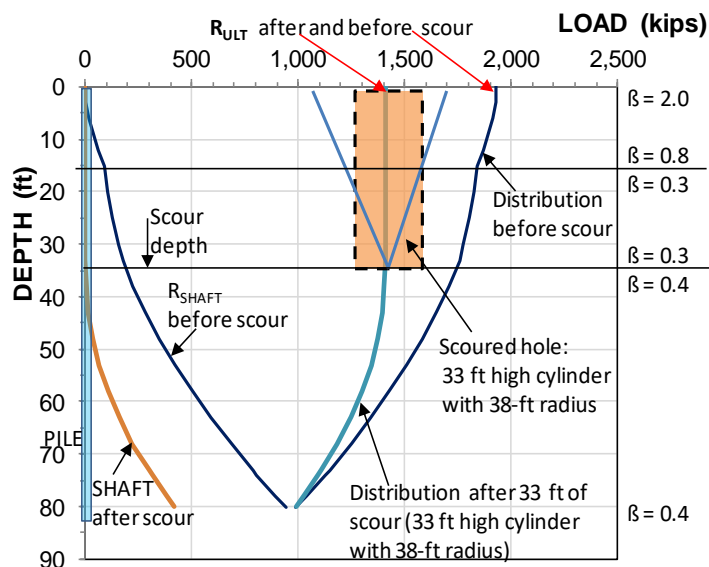
Fig. 7.64 Force distributions at "capacity" before and after-scour
