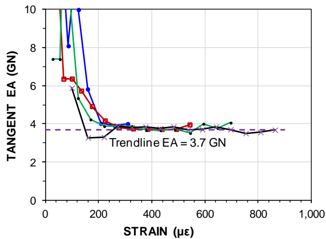
Fig. 8.78 Secant EA at L4
