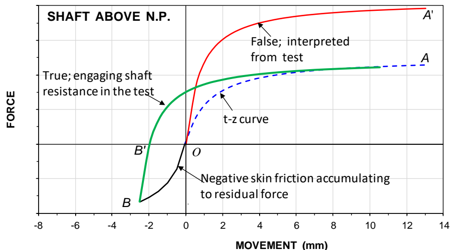
Fig. 8.35. The effect of "false" resistance from dowdrag developing before start of a static test.
