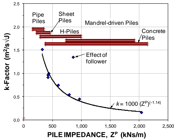
Fig. 9.24 Influence of pile impedance on the vibration factor, k (Eq. 9.30). (Data from Heckman and Hagerty 1978).
